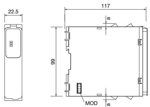
HR6S-EP形
