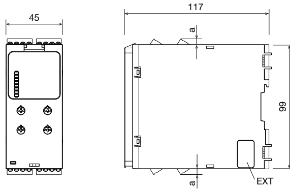
HR6S-AT形
