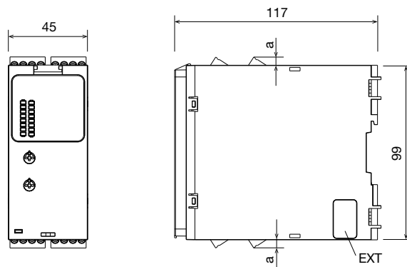
HR6S-DN形
